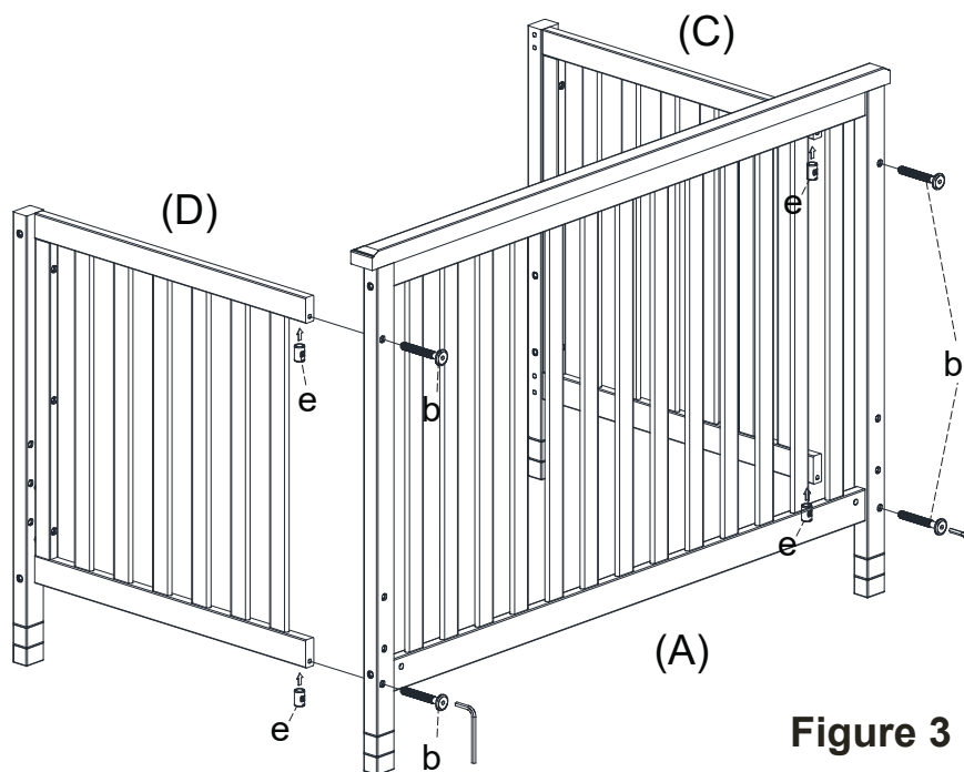
(b) M6 x 55mm Allen bolt (4 pcs)
